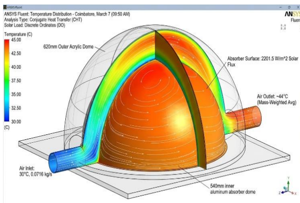
FIGURE 3. Three-Dimensional Flow Visualization Illustrating the Temperature Progression from Inlet (30°C) to Outlet Across the Aluminum Absorber.
