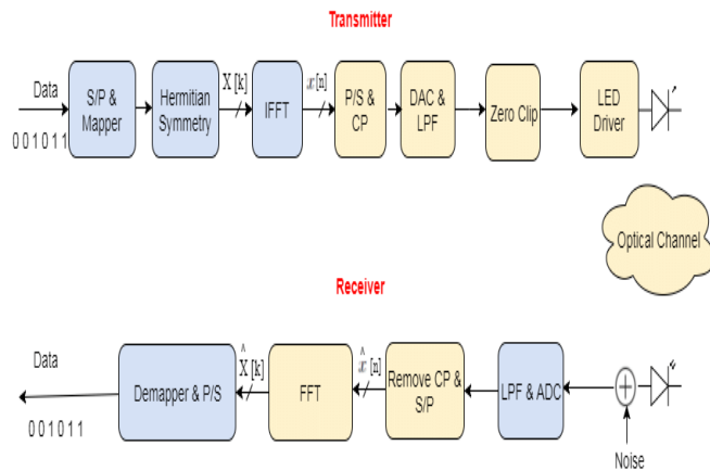
Figure 1 Block Diagram Of ACO-OFDM [1]
