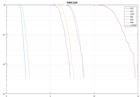
Figure 5 Graphical Representation of PAPR [5]
