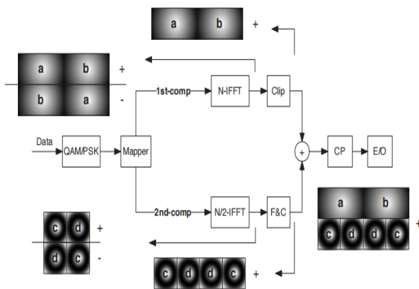
Figure 2 The Two-Component See-Ofdm Transmitter [2]
