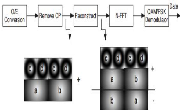
Figure 3 The Two-Component SEE-OFDM Reciever [3]
