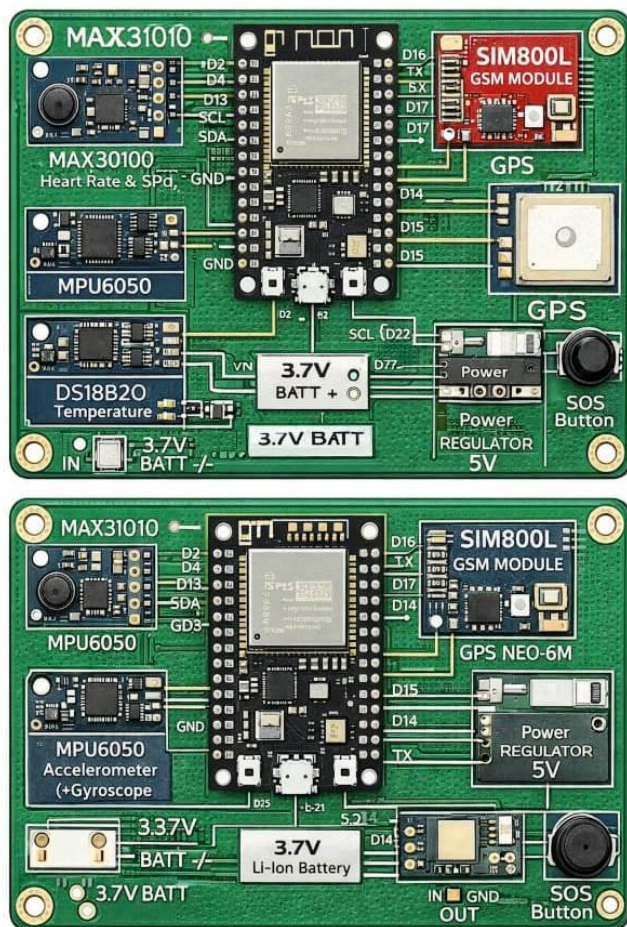
Figure 3 GSM Module
