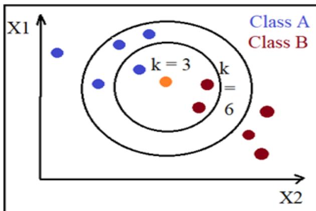
Figure 3 KNN Classifier [82-th]
